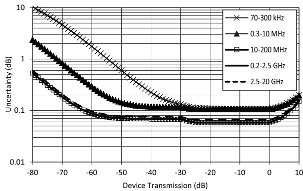
Transmission Magnitude Uncertainty; MS4642B (Opt. 61/62); 12-term Calibration using 36585K AutoCal
