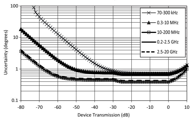
Transmission Phase Uncertainty; MS4642B (Opt. 61/62); 12-term Calibration using 36585K AutoCal
