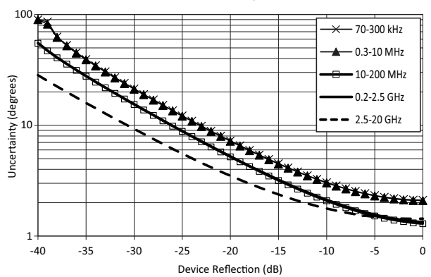
Reflection Phase Uncertainty; MS4642B (Opt. 61/62); 12-term Calibration using 36585K AutoCal
