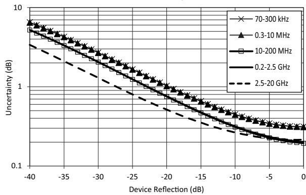
Reflection Magnitude Uncertainty; MS4642B (Opt. 61/62); 12-term Calibration using 36585K AutoCal
